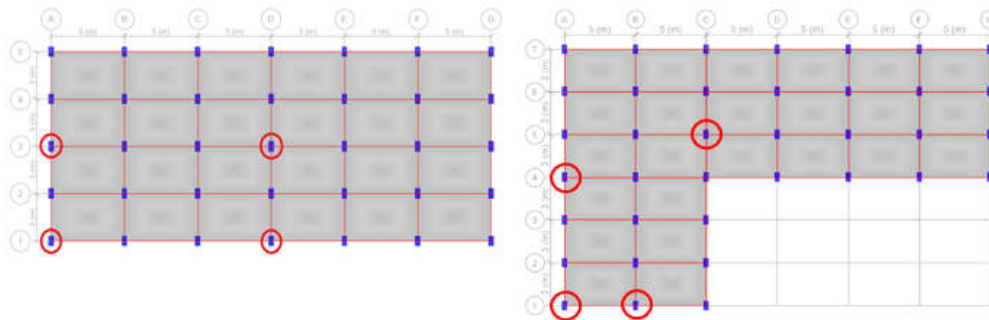
Figure 3. Plan and 3D model of L-shape Building Structure
