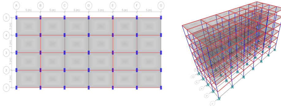
Figure 1. Plan and 3D model of Rectangular Building Structure
