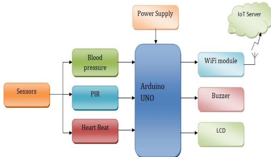
Fig.1 – Block diagram of healthcare system using IoT.
